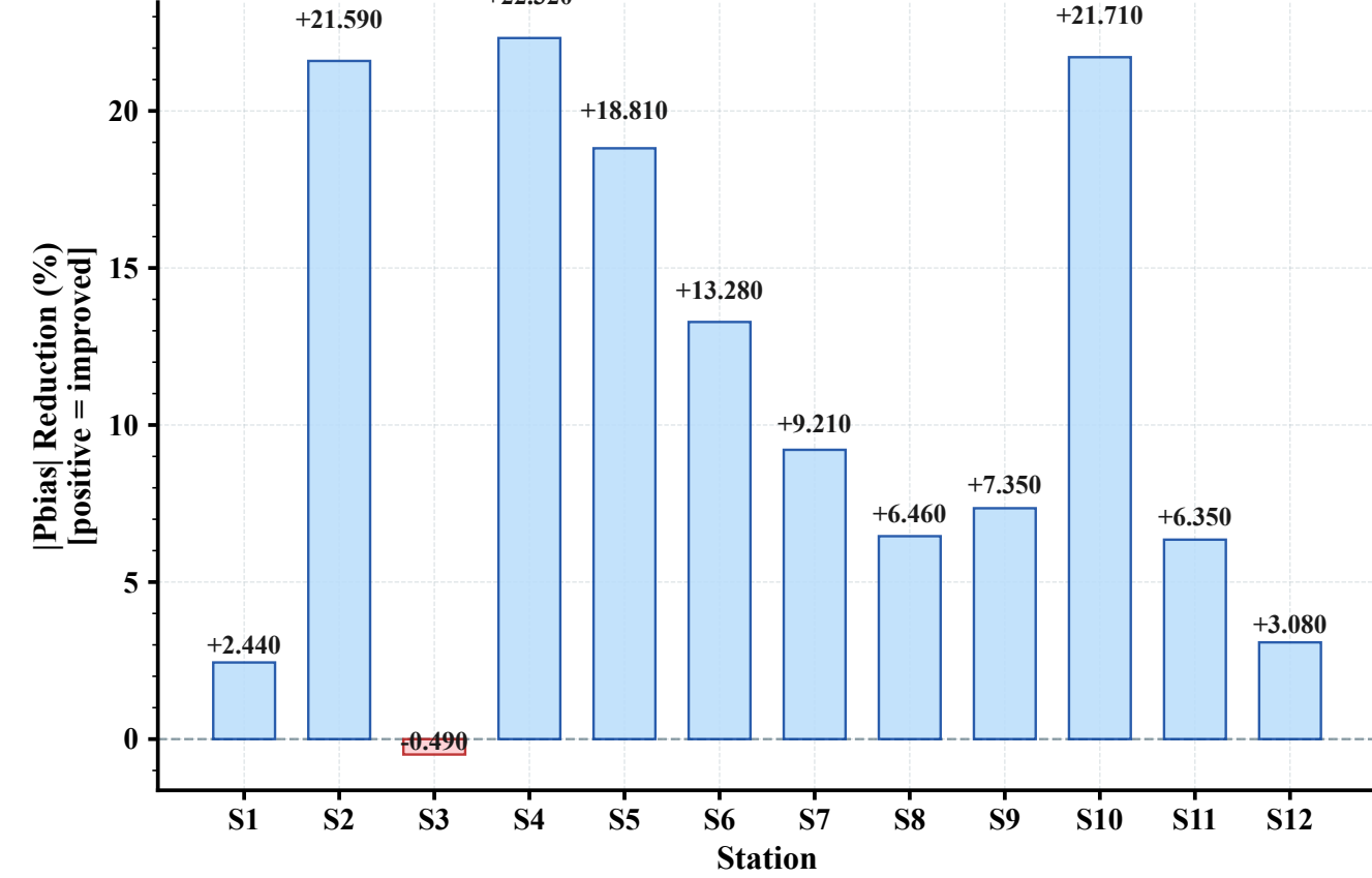
(b) Percent Bias Reduction
