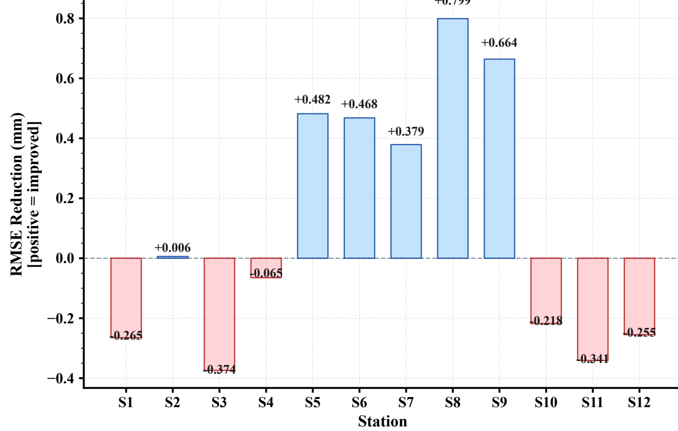
(a) RMSE Reduction After Bias Correction
